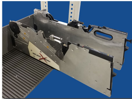
206 Cart Shown with E by SIPLACE and X Series Feeders
